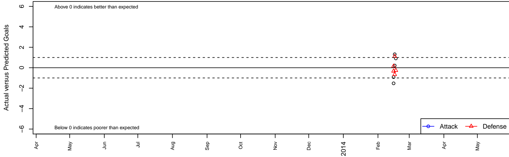
Rush Soccer SPI H B97 Dots are actual minus expected GF (blue circles) and GA (red triangles). Blue line is smoothed change in attack strength. Red is smoothed change in defense strength.
